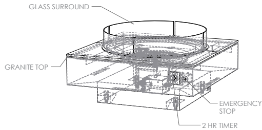
PERSPECTIVE VIEW
