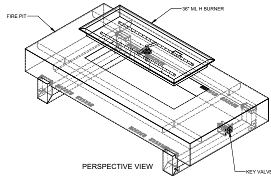
PERSPECTIVE VIEW
