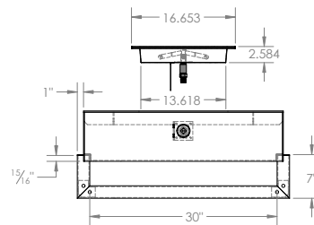
RIGHT VIEW
