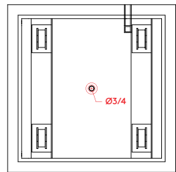
Drainage Fitting on Column with Casters and Irrigation Sleeve
