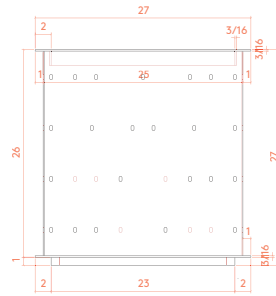
FRONT ELEVATION (PLANTER BODY)
