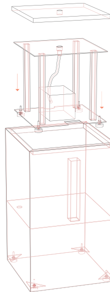
EXPLODED PERSPECTIVE
