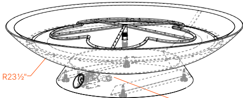
PERSPECTIVE VIEW
