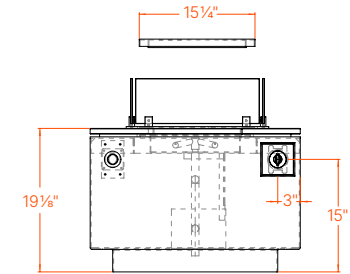
RIGHT VIEW
