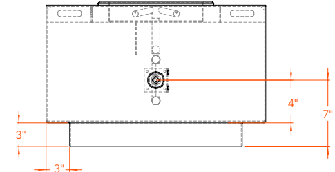
RIGHT VIEW
