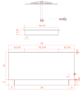
CSA Certified Pento Burner Natural Gas - 65k BTU 120VAC
