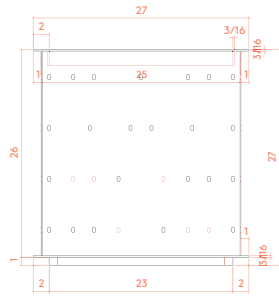
FRONT ELEVATION (PLANTER BODY)
